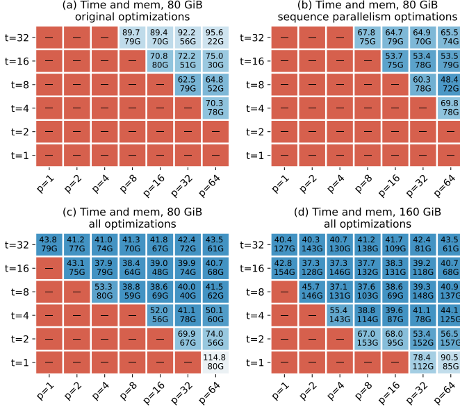
Figure 5: Batch time training with various optimizations and constraints (dashes indicate infeasible configurations due to a lack of memory). The top number shows the best batch time, and the bottom number shows the required memory to run, t and p measure the degree of TP and PP. (a) time for a system with 32 A100 with 80 GiB HBM in a single NVLink domain and original optimizations set [29]; (b) same with partial recompute and sequence parallelism [20]; (c) same with all optimizations from Table 1; (d) same with memory capacity increased to 160 GiB per GPU.
