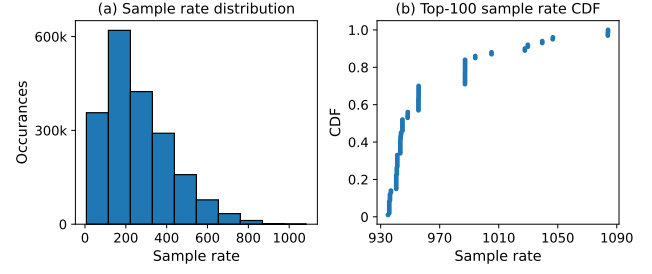
1,974,902 execution strategies for GPT3 175B on 4096 GPUs
