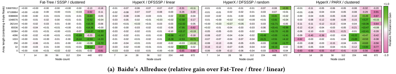
Figure 4: Relative performance gain compared to Fat-Tree / ftree / linear combination (cf. Sec. 4.4.3) for various MPI collectives
