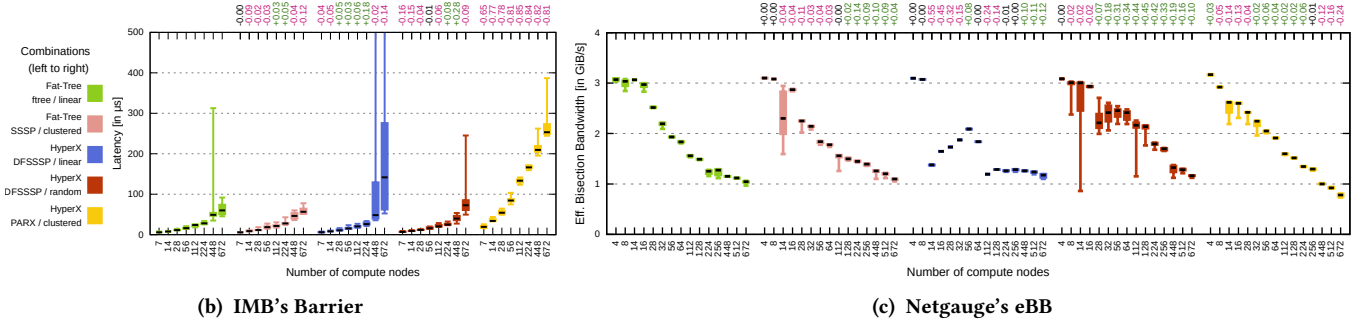
Figure 5: Rest of network benchmarks; Whisker plots for 10 runs show in Fig. 5b and 5c (numbers above each Figure indicated relative performance gain over Fat-Tree / ftree / linear for the best run of both combinations); See Sec. 5.1 for detailed analysis
